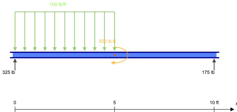
Free Body Diagram (FBD)
