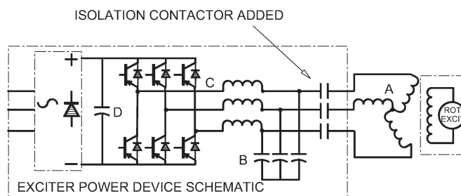
Fig. 2. Exciter controller to motor interface.
