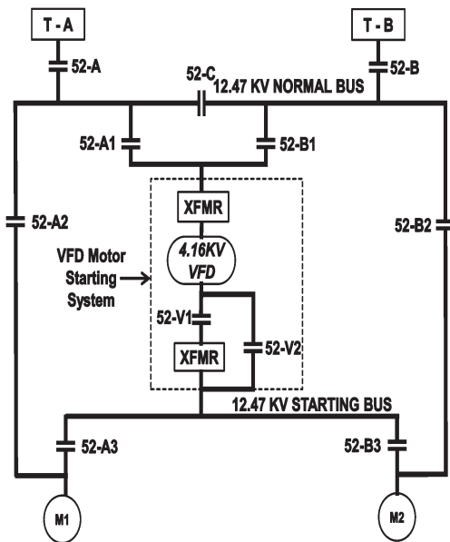
Fig. 3. Starting VFD system: Example for two motors.
